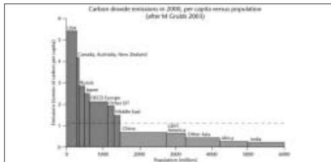
Figure 3. Carbon dioxide emissions in 2000 per capita for different countries and groups of countries 14 . The global per capita average is shown by the dotted line.
