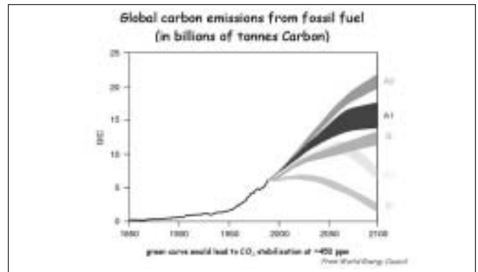
Figure 2. Global emissions of carbon dioxide from fossil fuel burning (in billions of tonnes of carbon) up to 1990 and as projected to 2100 under World Energy Council scenarios 9 . The A and B curves refer to various 'business as usual' assumptions and Curve C is the 'ecologically driven scenario' that would lead to stabilization of carbon dioxide concentration at about 450 ppm.
